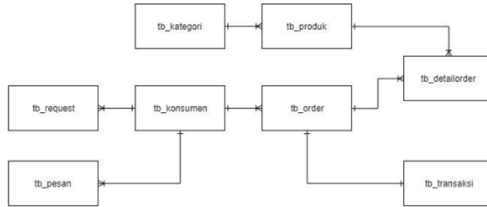
Gambar 5. Entity Relationship Diagram (ERD) Crow's Foot Model
