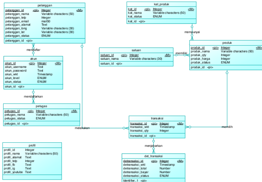
Gambar 3. Conceptual Data Model E-commerce De Janggelan
