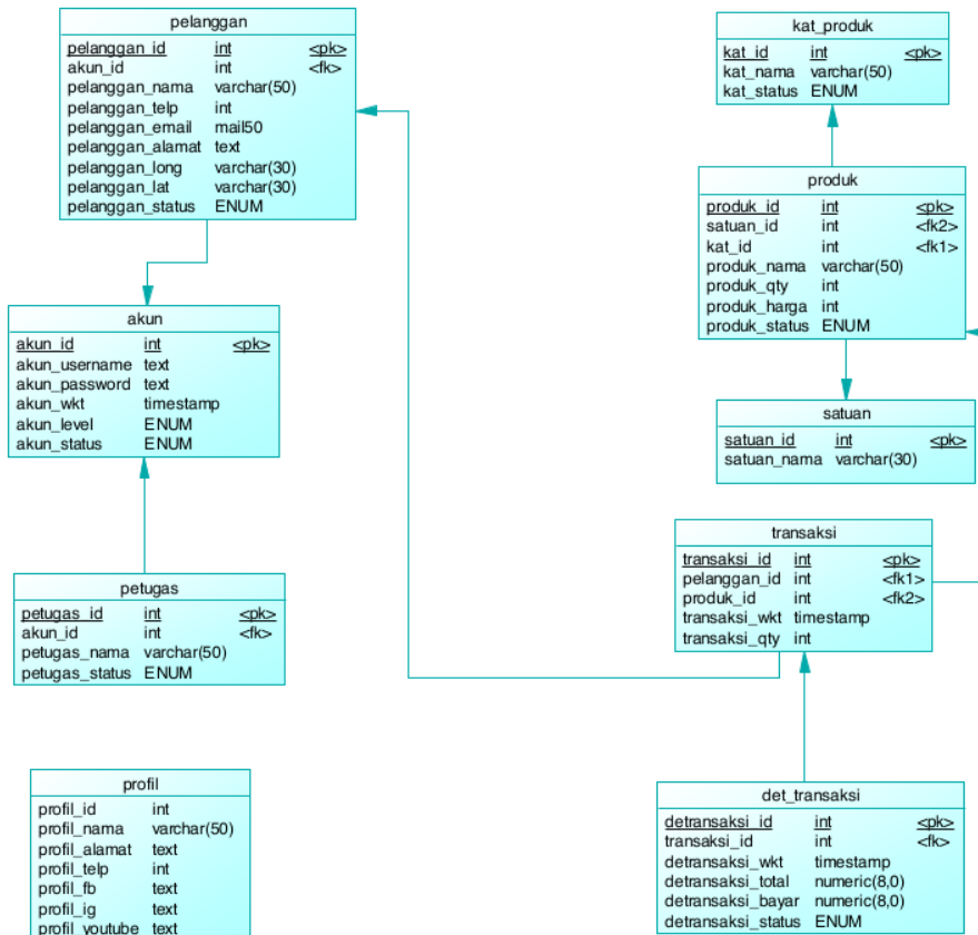
Gambar 4. Logical Data Model E-commerce De Janggelan
