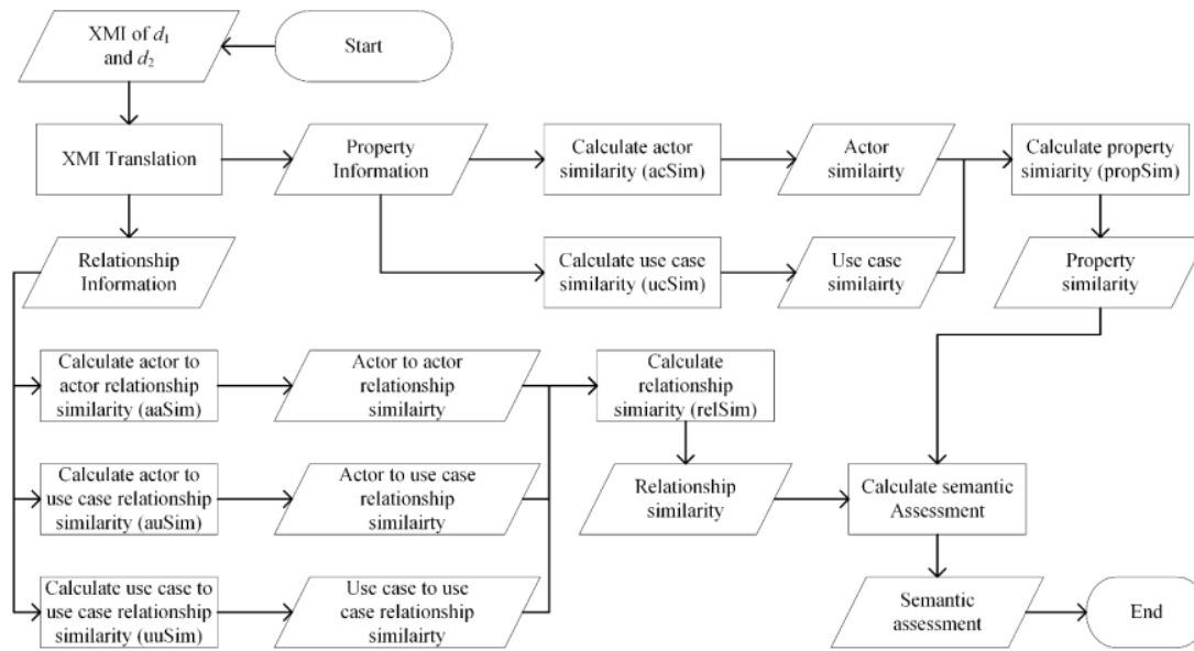
Figure. 4 Flowchart of semantic assessment
