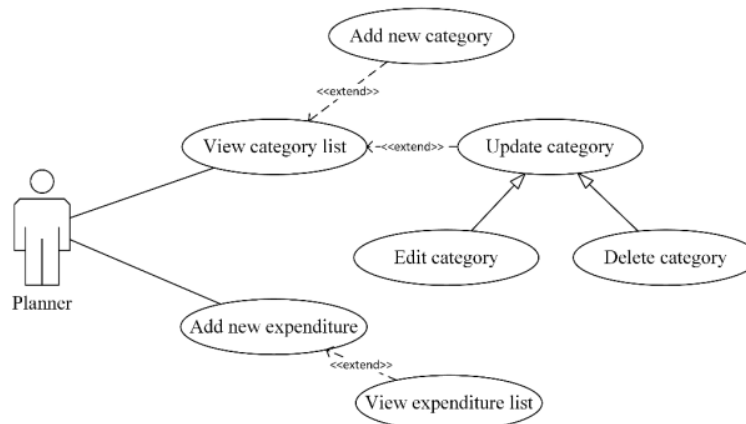
Figure. 2 Example of use case diagram (Outlay)
