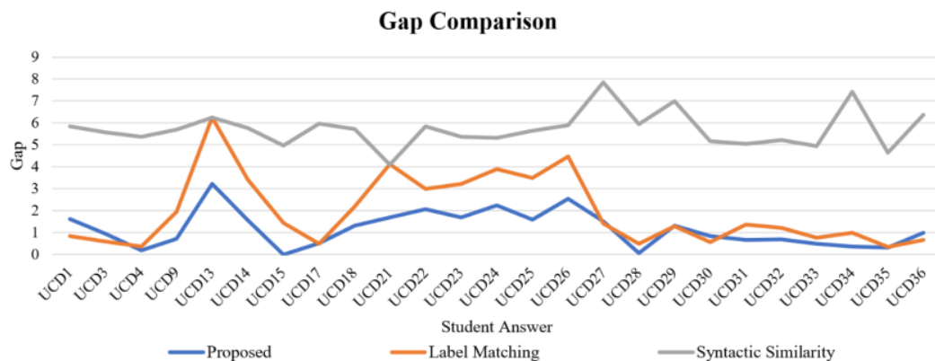
Figure. 7 Comparison with previous research
